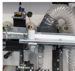
PRE-MILLING UNIT
